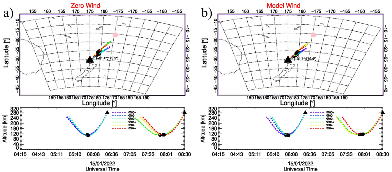
Figure A1. Backward ray paths of the medium-scale TIDs observed over New Zealand as a function of longitude and latitude (upper panel), and as a function of time and altitude (lower panel). Reverse ray tracing was run in both zero (a) and model (b) wind mode. For the ray tracing, we use the MSTIDs parameters observed over New Zealand from Table 1. The light pink dot indicates the location of the Tonga volcano eruption. The black triangles and dots indicate where the ray tracing started and where the GW upward reflected on the trace path, respectively. The colored lines correspond to the individual ray path of the waves (NZ03 and NZ04). Note that each LSTID has three paths because we are considering the ray paths of the mean LSTID parameters (NZ), the mean parameters plus standard deviation (NZ+), and the mean parameters minus standard deviation (NZ−).
