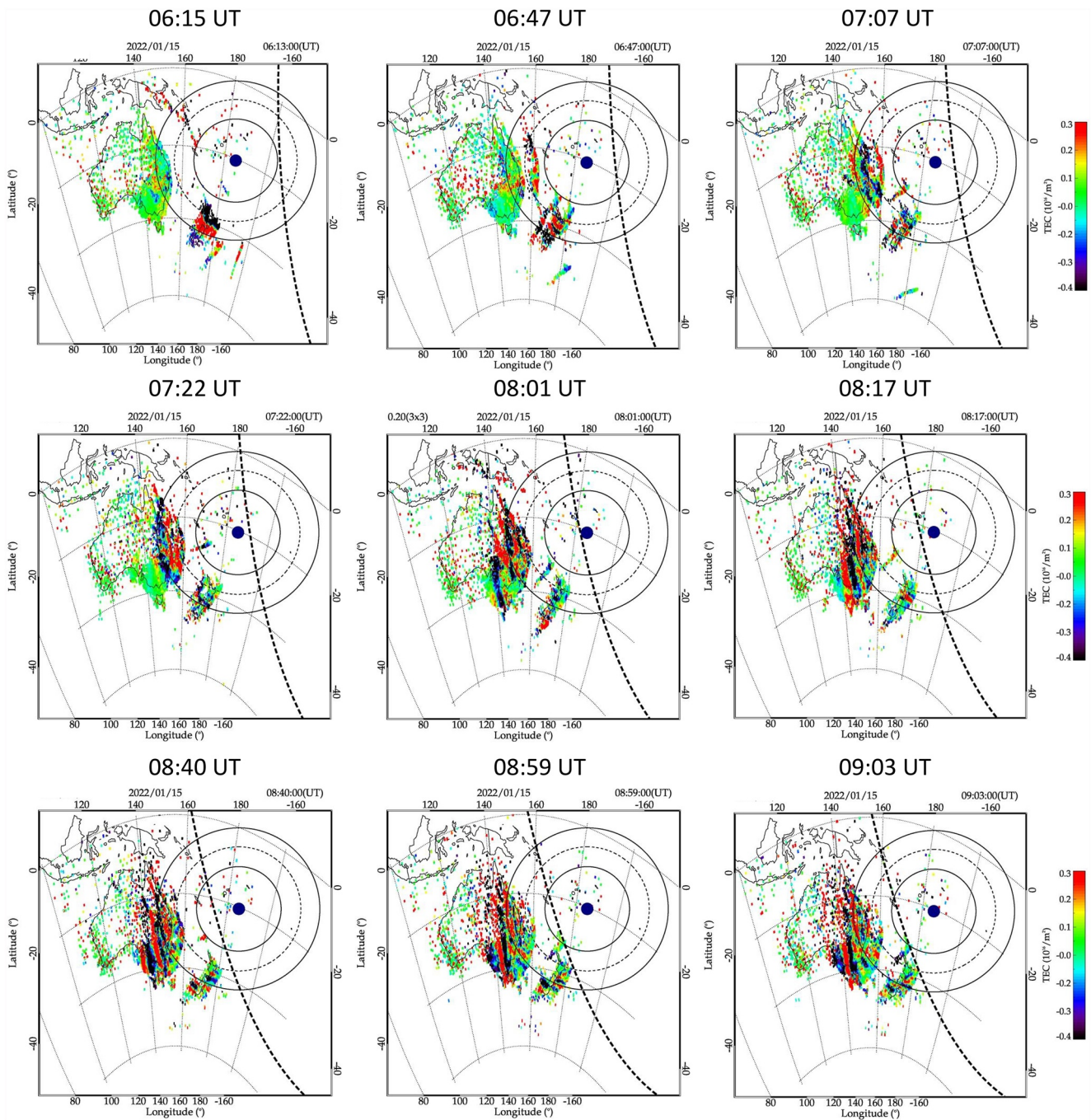
Figure 2. Detrended TEC maps over Australia and New Zealand during the Tonga volcanic eruption on 15 January 2022 from 06:13 to 09:03 UT. Alternating red and black colors indicate the TIDs generated by the Tonga eruption. The Tonga volcano is located at the blue dot. The inner to outer circles indicate the radii of 2,000, 3,000, and 4,000 km, respectively, from Tonga. The dashed black lines represent the dusk solar terminator at \sim 300 km height. The color scale is in accordance with the disturbance signal, from red (positive) to black (negative).
